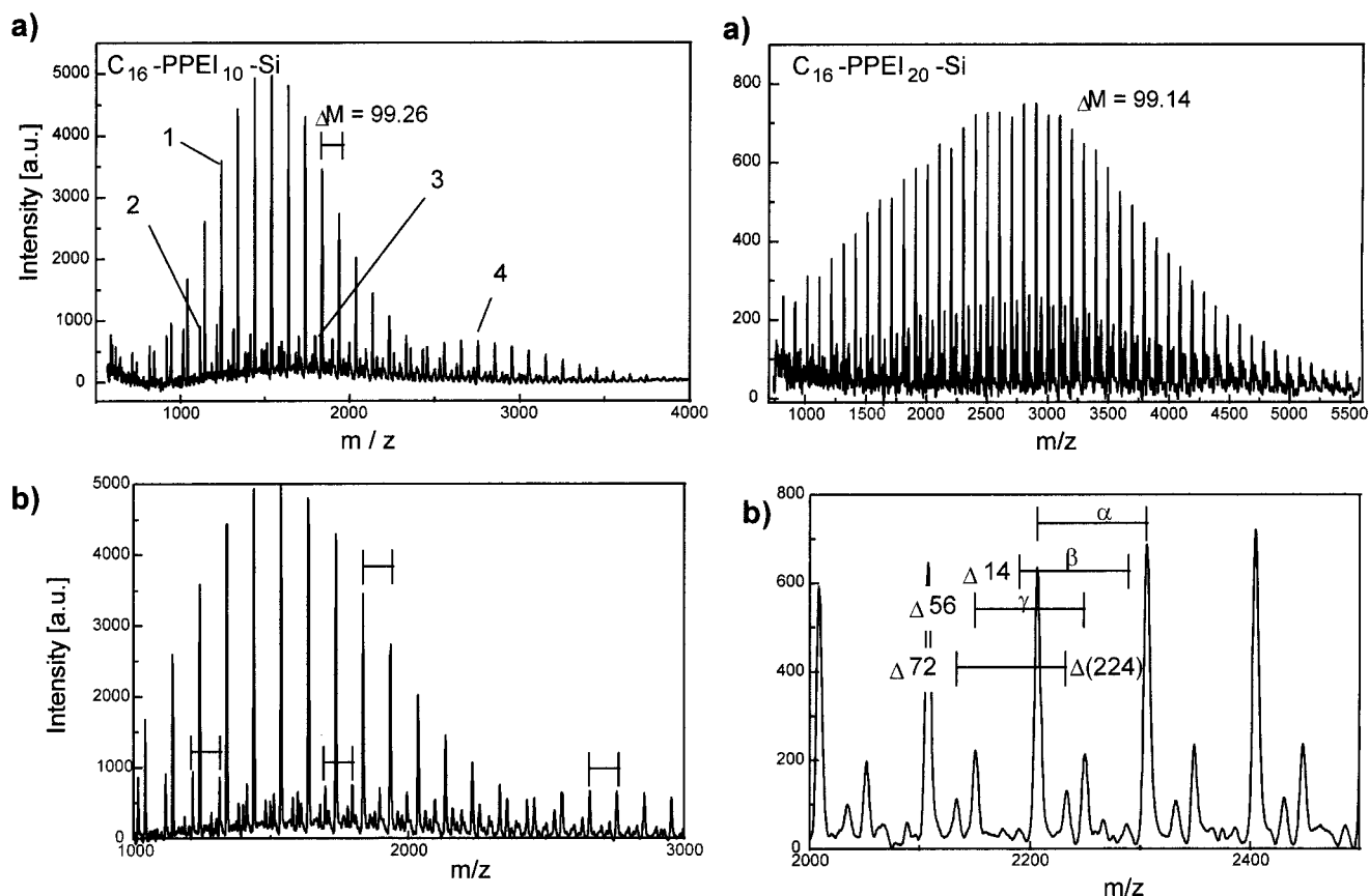
Figure 5. MALDI TOF MS spectrum of C 16 -PPEI n -Si with n = 10 (a, left) and n = 20 (a, right) along with a detailed view (b).
