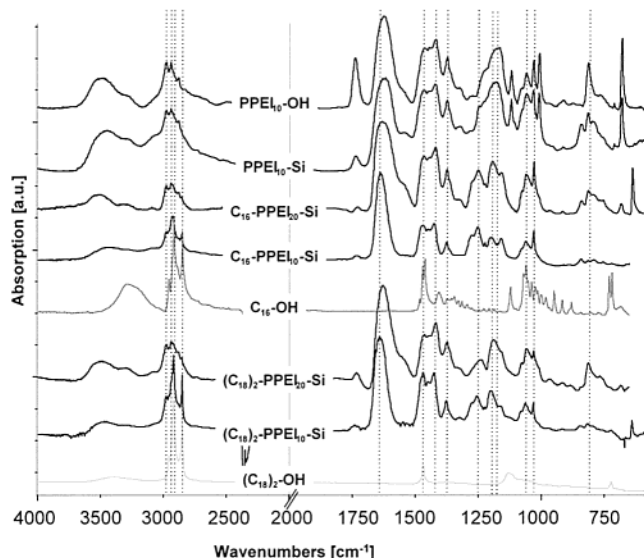
Figure 3. Transmission FTIR spectra of all polymers in the spectral range from 4000 to 600 \text{cm}^{-1} . For better comparison the spectra of the alcohols used for the initiators are depicted (gray lines). For exact positions of band maxima refer to Table 2.
