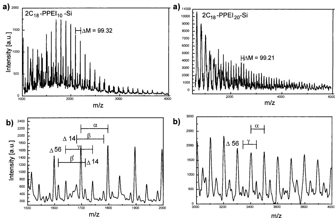
Figure 6. MALDI TOF MS spectrum of (C_{18})_2\text{-PPEI}_n\text{-Si} with n = 10 (a, left) and n = 20 (a, right) along with a detailed view (b).
